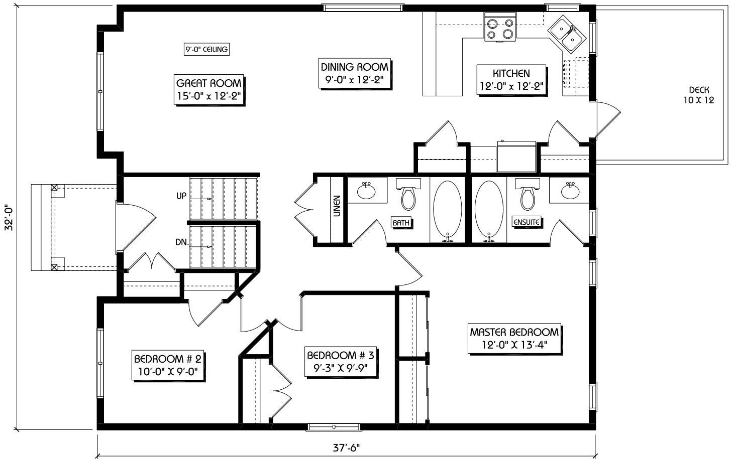
MAIN FLOOR PLAN 1182 SQ. FT.
